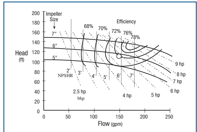
Figure 13. Performance Curves for a 4x1.5-6 Pump Used for Water Service
