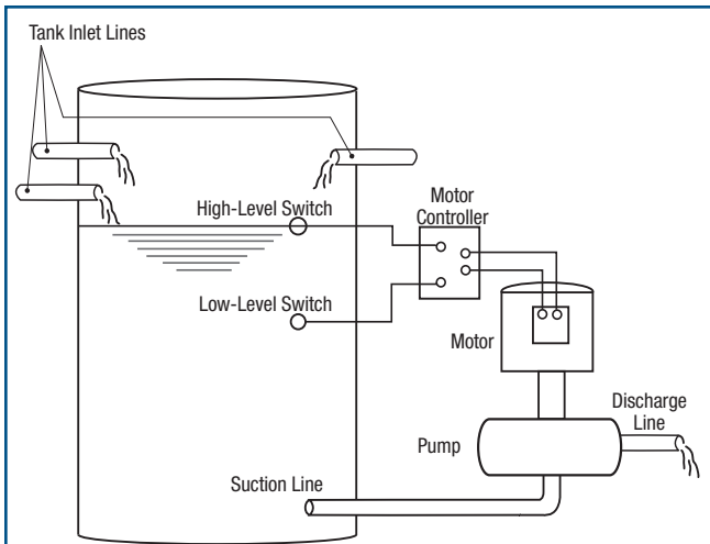
Figure 16. Typical Tank Level Control
