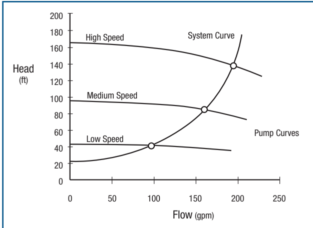
Figure 15. Multiple-Speed Pump Performance Curves
