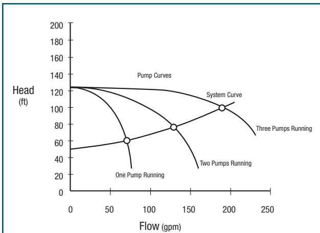
Figure 14. Multiple Pump Operation
