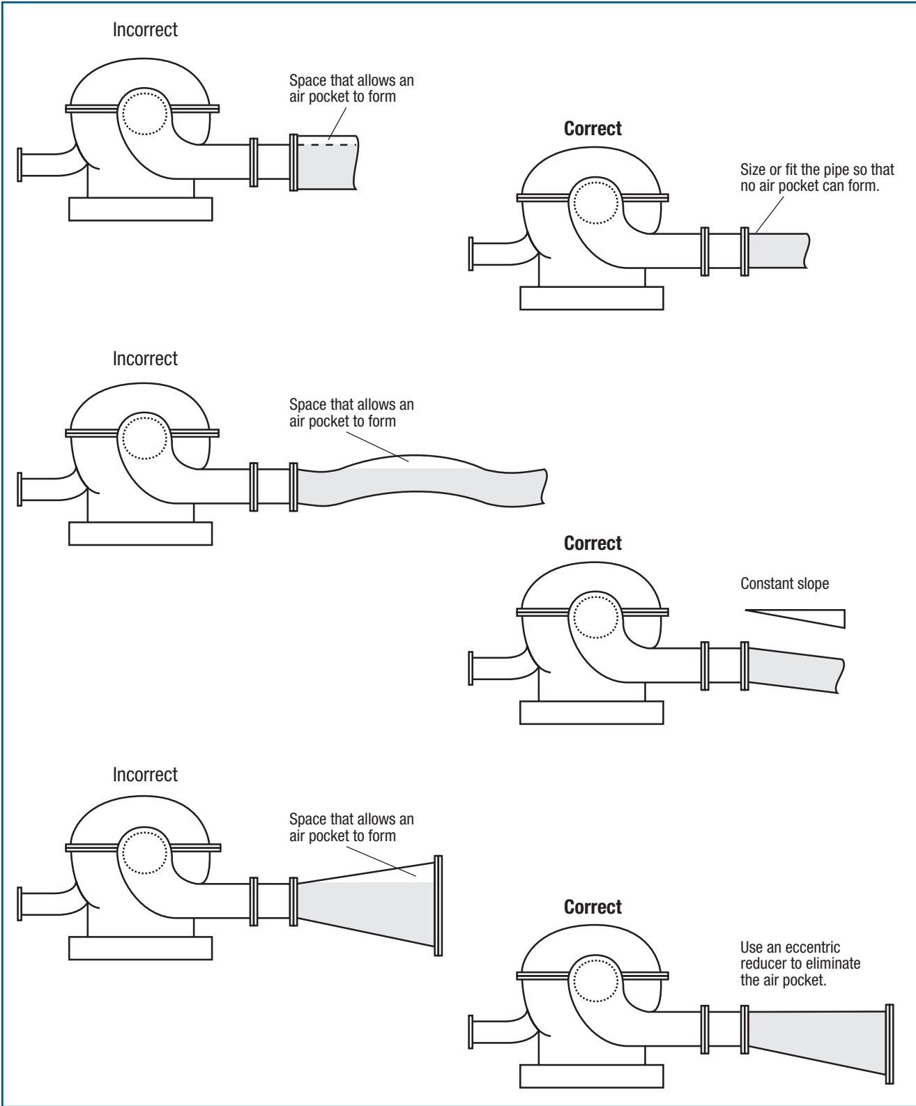
Figure 7. Common Pipe Configuration Problems and How To Correct Them
