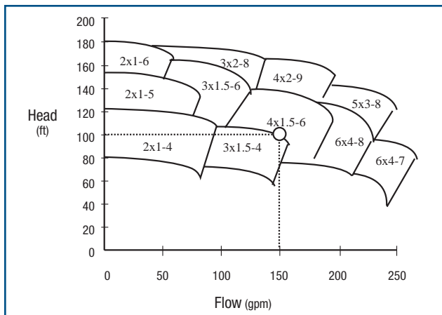
Figure 11. Family of Pump Performance Curves
