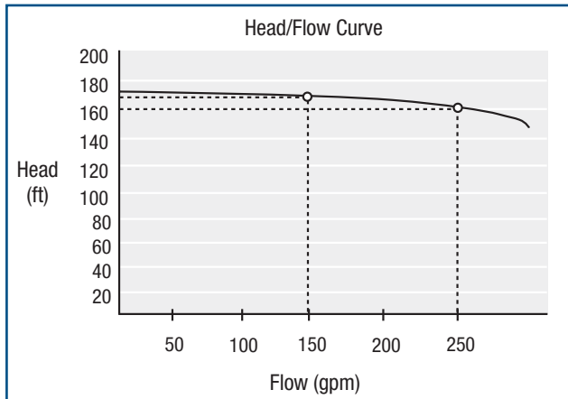
Figure 3. Illustration of the Sensitivity of Flow to Changes in Backpressure
