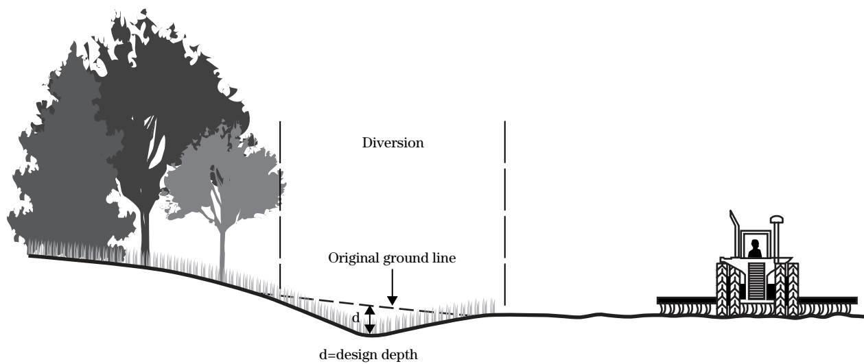
Figure 9-3 Channel diversion
