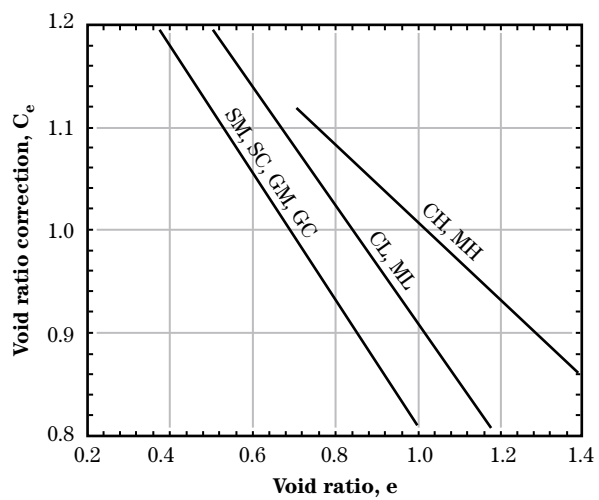
Figure 9-8 Correction for void ratio
