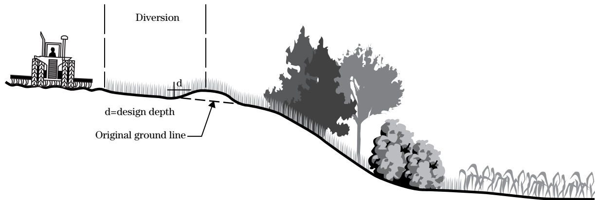
Figure 9-2 Ridge diversion
