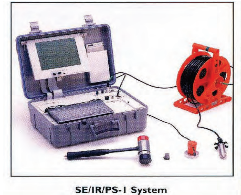
Figure 11.3.42 Parallel Seismic Testing Equipment
