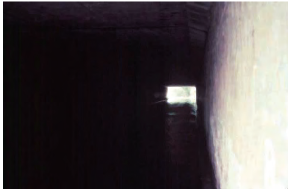
Figure 7.12.7 Sighting Along Culvert Sidewall to Check Horizontal Alignment
