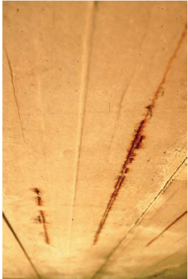
Figure 7.10.18 Burlap Fold Depressions in an Early 1950's P/S Box Beam
