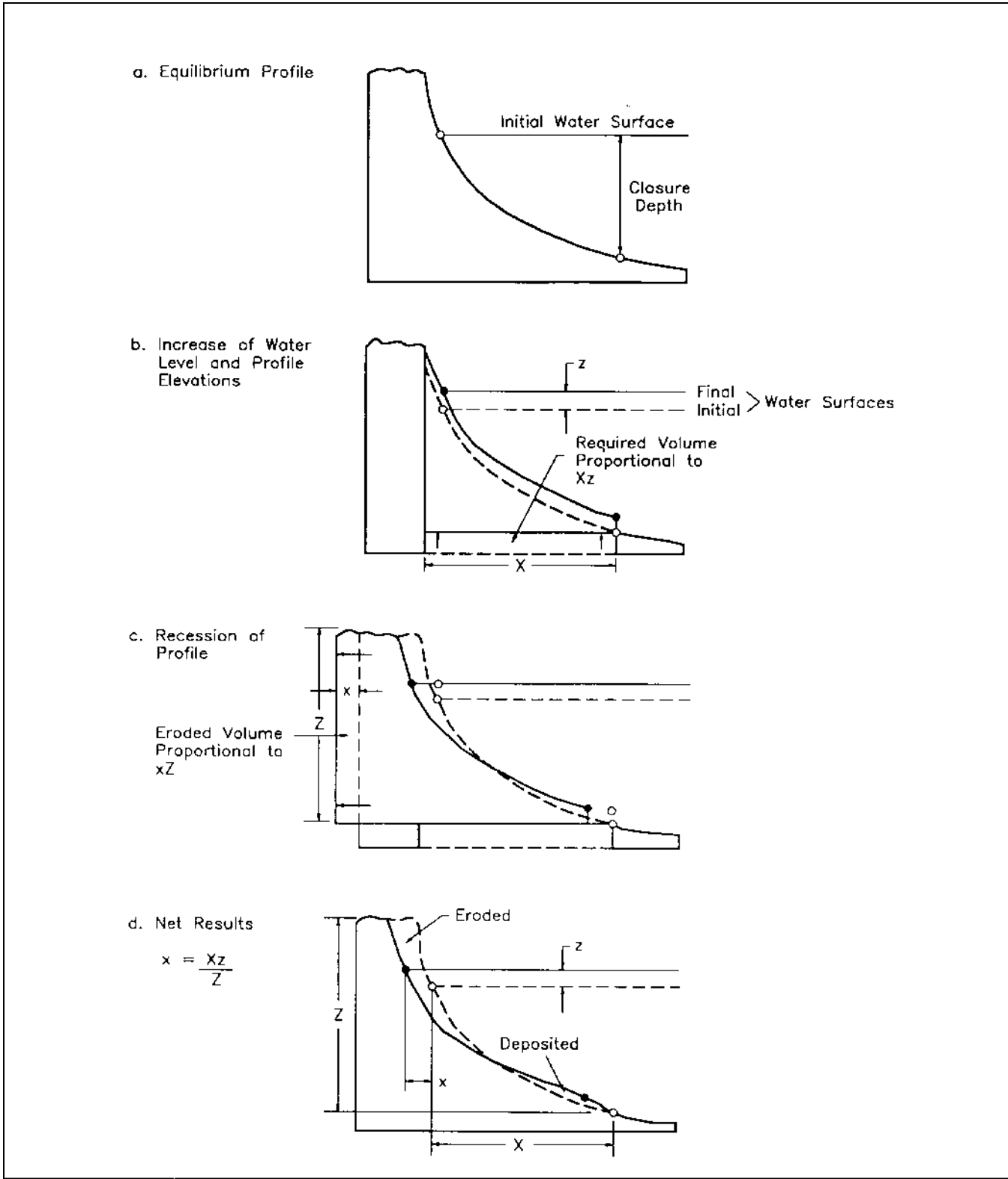
Figure 4-28. Profile adjustment in two stages, first vertical, then horizontal, demonstrating the basis for the Bruun Rule (Equation 4-6) (from Hands (1983)). Details are discussed in the text
