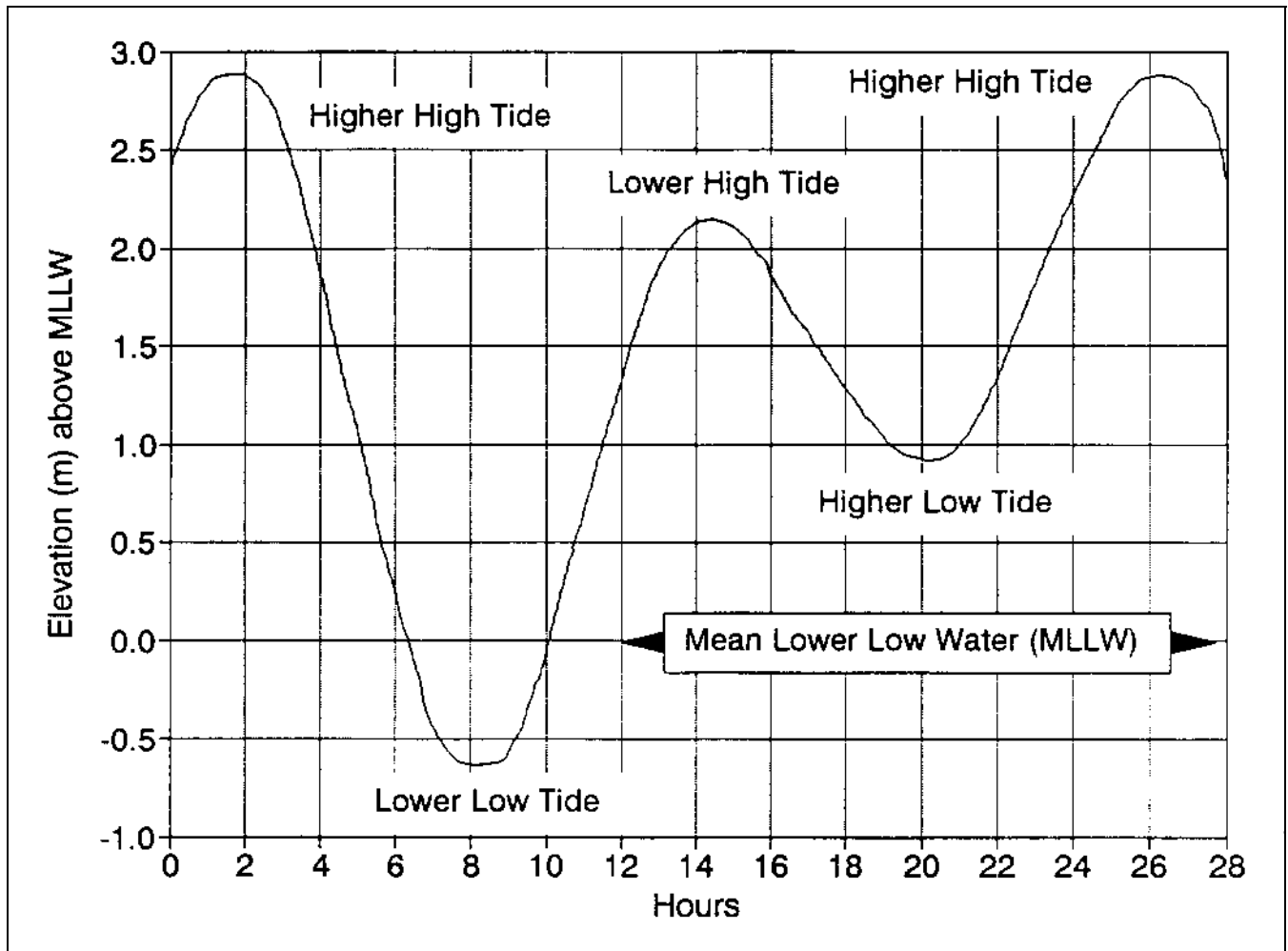
Figure 2-4. Tide curve for Yaquina Bay, Oregon (based on 6 years of observations). By definition, mean lower low water (mllw) is zero (from Oregon (1973))
