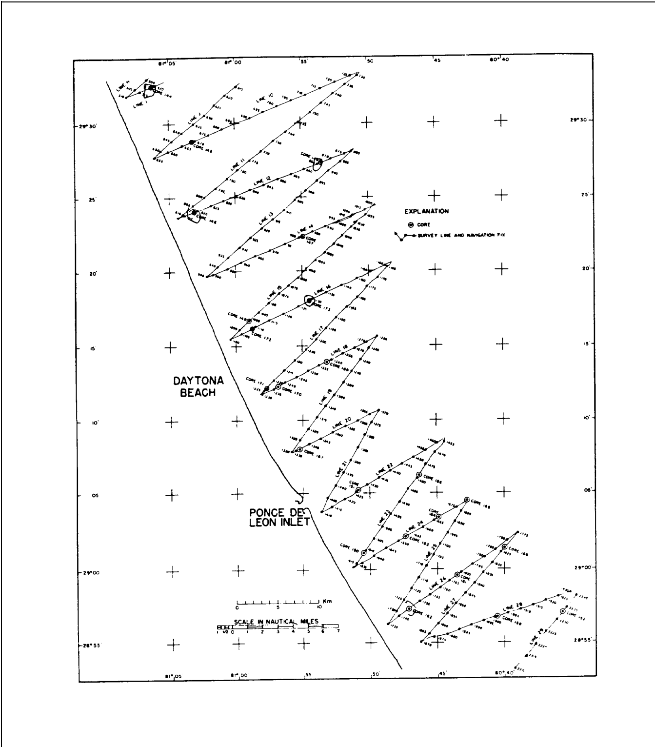
Figure I-2. Zigzag reconnaissance survey pattern from the Florida east coast (from Meisburger (1990)) 1
