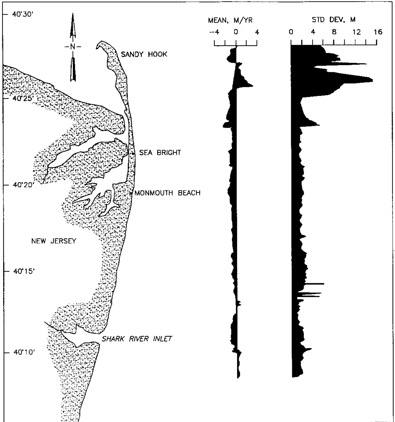
Figure 5-28. Distinctive spatial shoreline trends along the northern New Jersey shore
