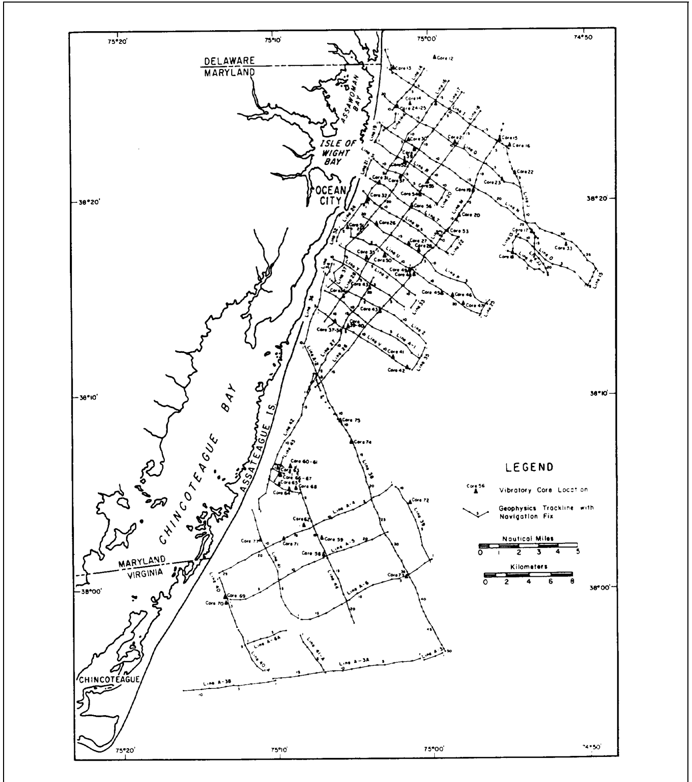
Figure I-1. Rectangle grid survey pattern used by Field (1979) off the Delmarva Peninsula
