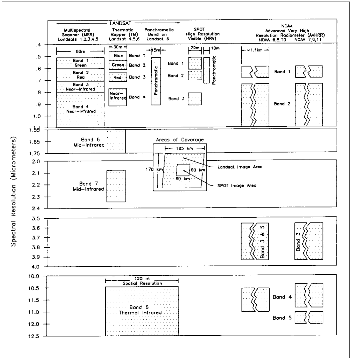
Figure 5-4. Spectral resolution and approximate spatial resolution of sensors on Landsat, SPOT, and NOAA satellites (from Earth Observation Satellite Company literature and Huh and Leibowitz (1986))
