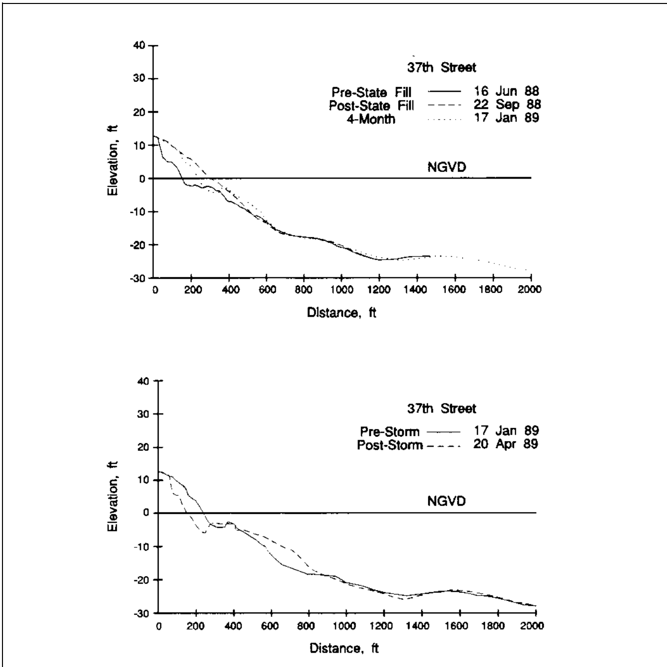
Figure 5-31. Analysis of the Ocean City, MD, beach fill project. Upper plot shows profile before beach fill and the large quantity of sand placed on the beach during the summer of 1988. Lower plot shows erosion of the upper profile during a storm in early 1989. Sand from the beach moved offshore to the region between 400 and 900 ft from the benchmark
