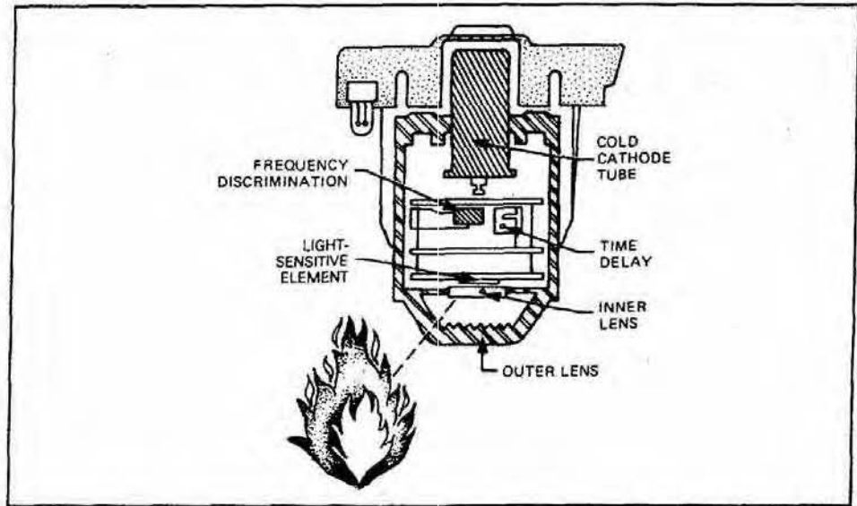
Figure VI-6. Infrared radiation detector. A light sensitive element attached to a frequency discriminating device is used to sense infrared radiation.
