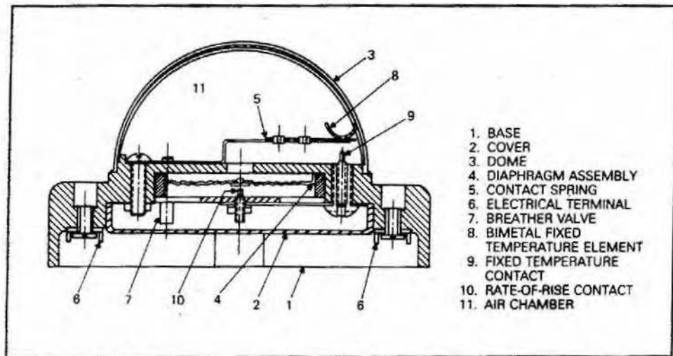
Figure VI-5. Combination heat detector.
