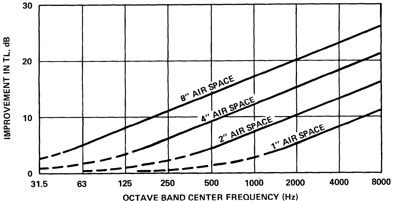
Figure 4-1. Improvement in Transmission Loss Caused by Air Space Between Double Walls Compared to Single Wall of Equal Total Weight, Assuming no Rigid Ties Between Walls.
