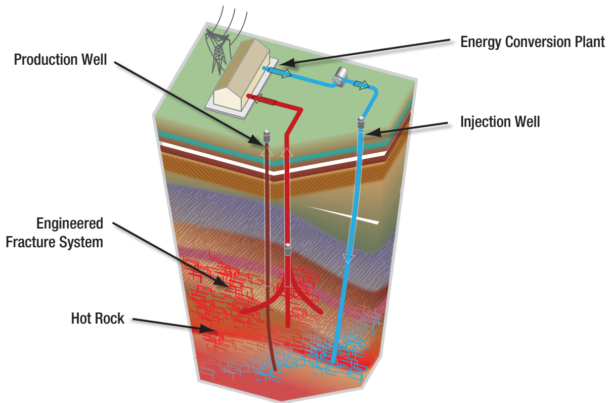
Figure 2. EGS Cutaway Diagram
