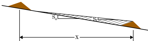
Figure TS14G-19 Spacing of grade control structure
