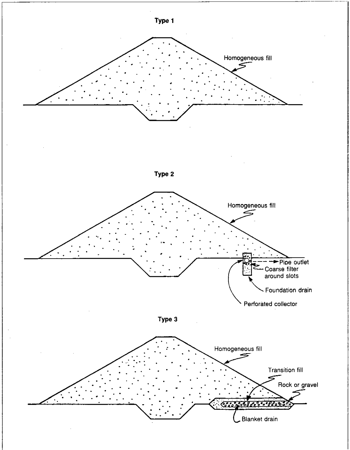
Figure 4-15.—Embankment types.
