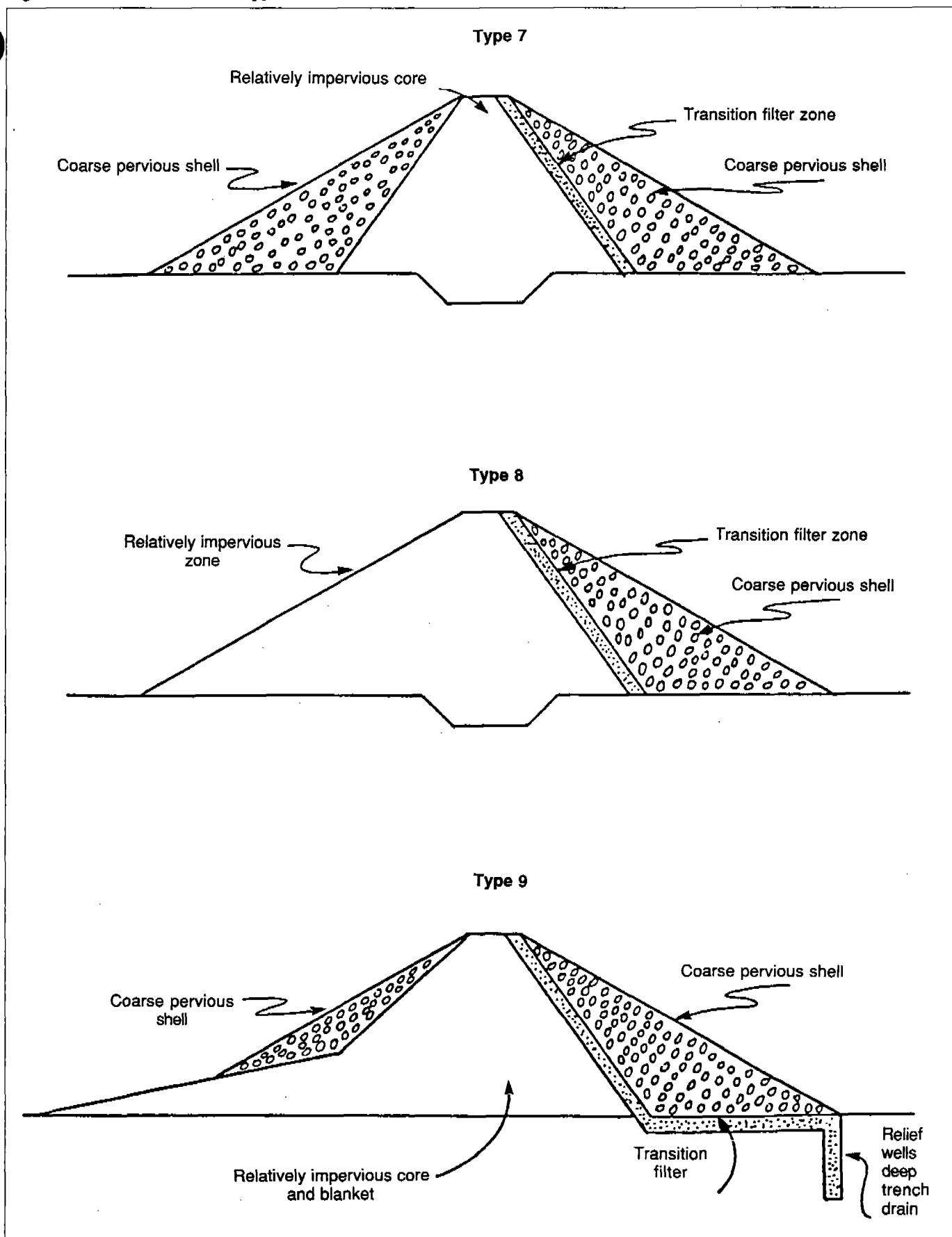
Figure 4-15.—Embankment types — Continued.
