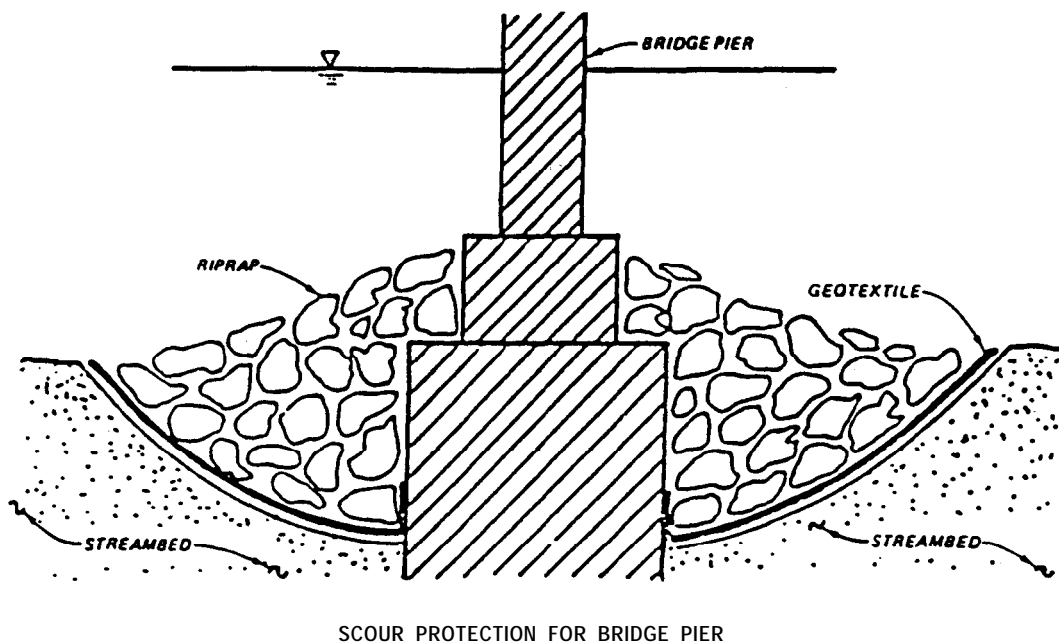
Figure 6-6. Use of Geotextiles around Piers and Abutments.
