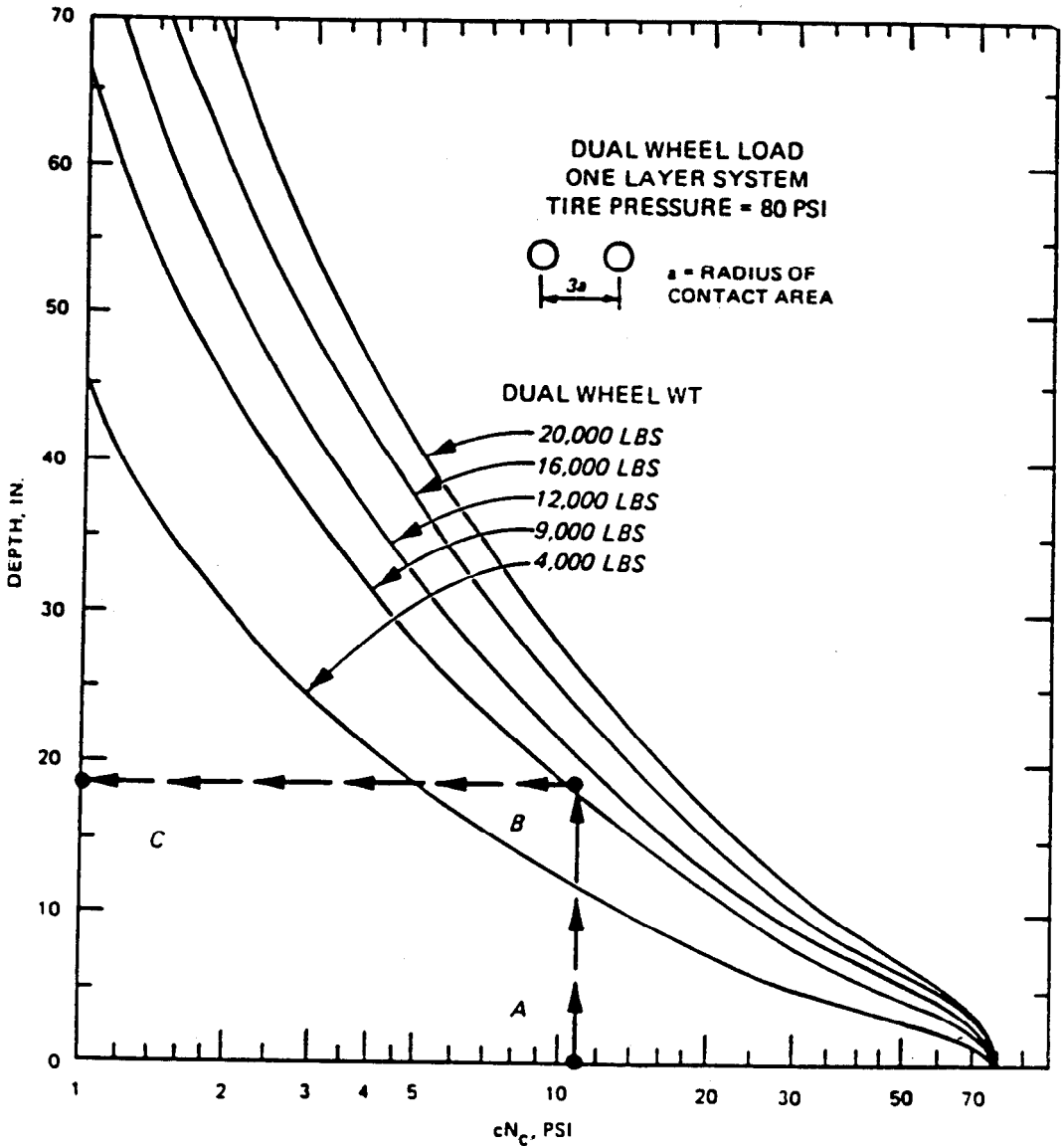
Figure 2-5. Thickness Design Curve for Dual-Wheel Load on Gravel-Surfaced Roads.
