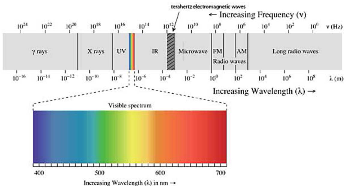
Figure 4-1 Electromagnetic (EM) Spectrum
