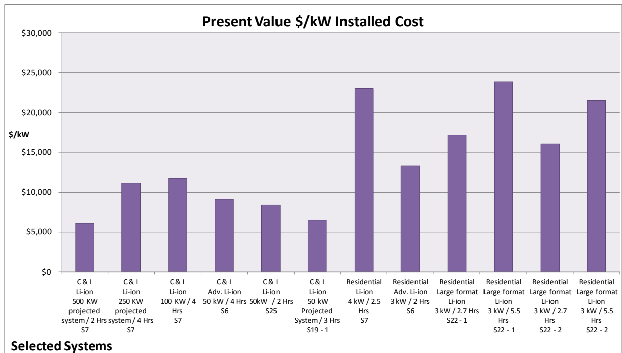
Figure 110. Present Value Installed Cost in $/kW for Li-ion Batteries in Commercial and Industrial Applications
