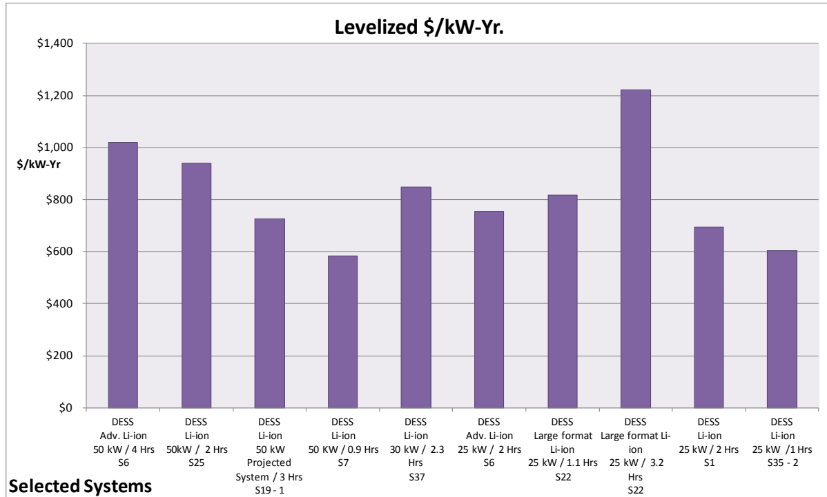
Figure 109. Levelized $/kW-yr for Li-ion Batteries in Distribute Energy Storage System Applications
