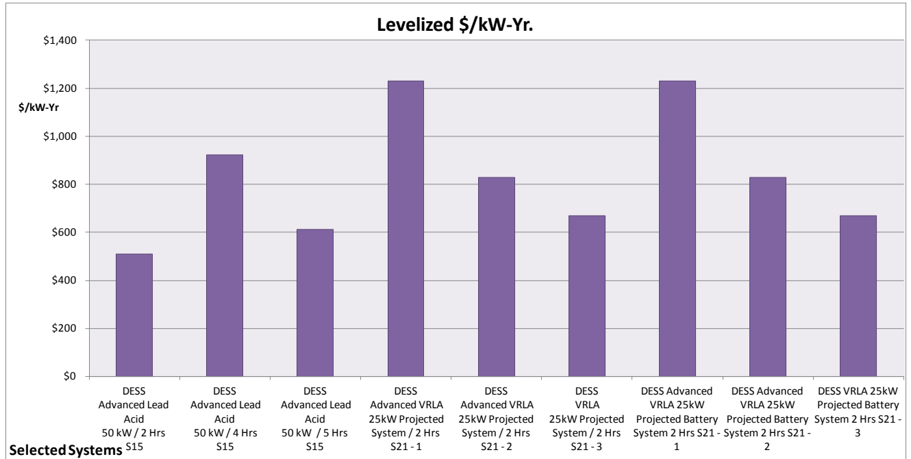
Figure 85. Present Value Installed Cost and Levelized Costs in $/MWh and $/kW-yr for Lead-acid Batteries in Distributed Energy Storage System Applications
