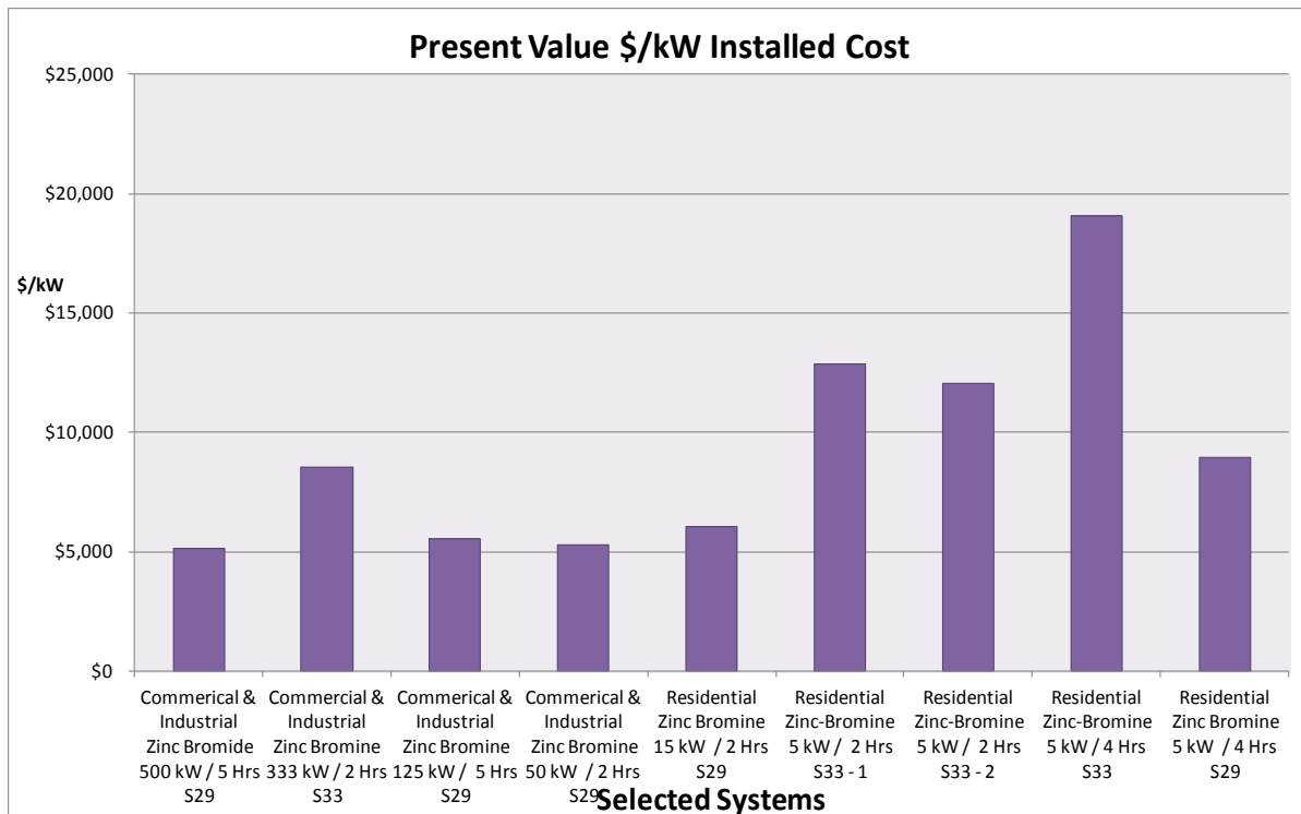
Figure 61. Present Value Installed Cost for Zinc-bromine Systems in Commercial and Industrial and Residential Applications
