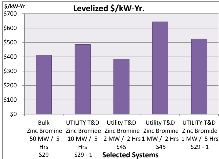
Figure 60. Levelized Cost of Capacity in $/kW-yr for Zinc-bromine Systems in Bulk and Utility Transmission and Distribution Service
