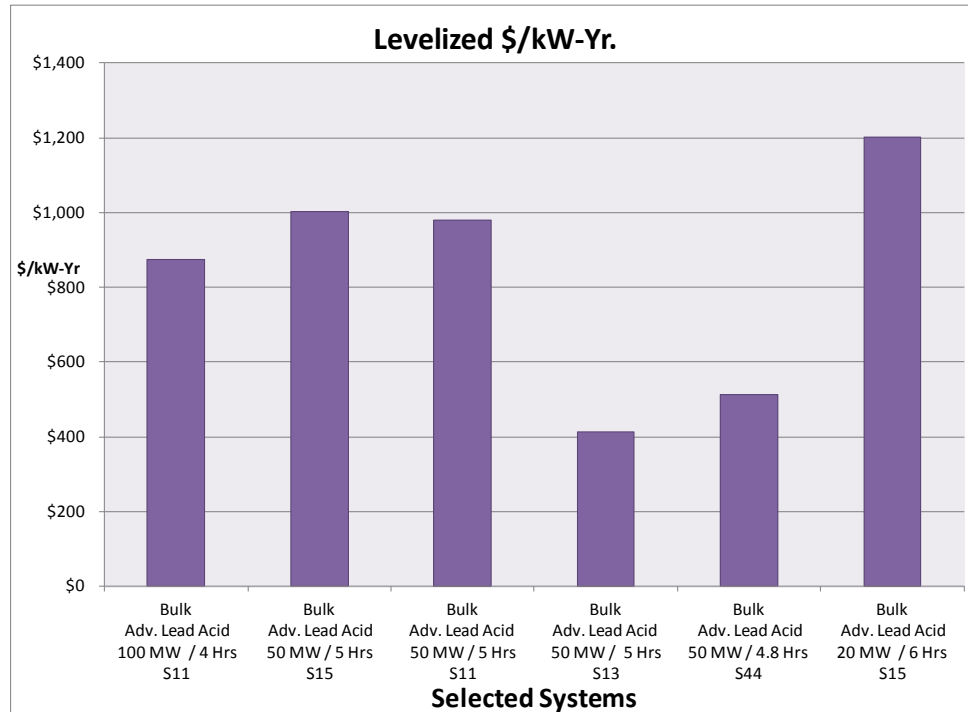
Figure 76. Present Value Installed Cost and Levelized Costs in $/MWh and $/kW-yr for Lead-acid Systems in Bulk Service Applications
