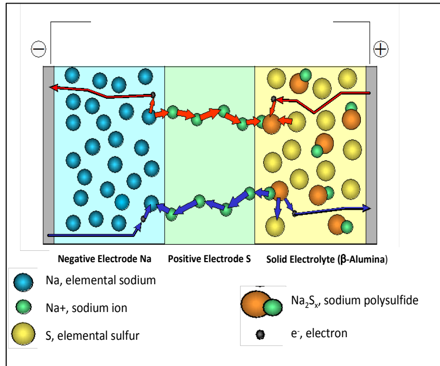
Figure 32. Chemical Structure of a Sodium-sulfur Cell
