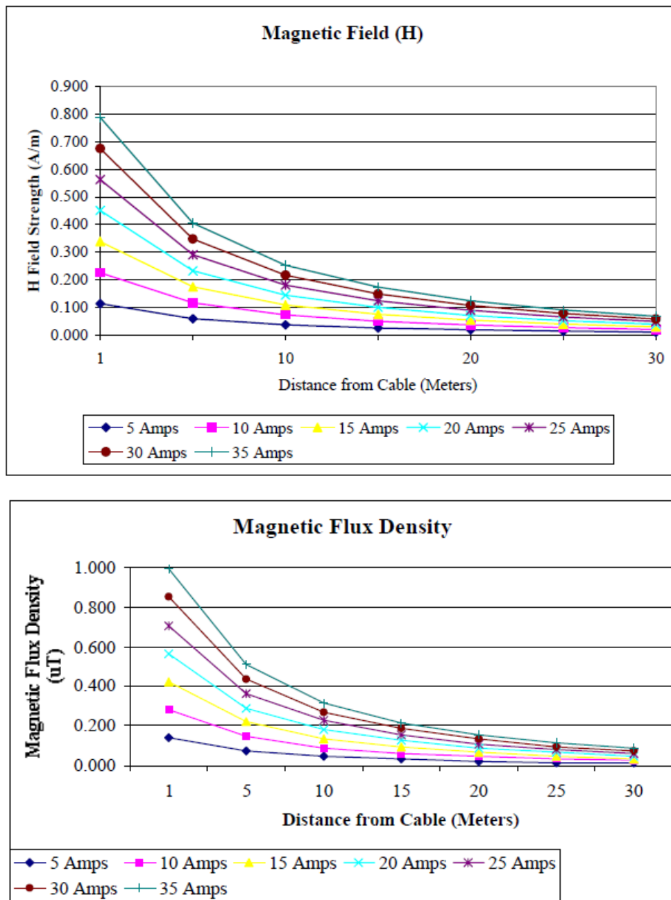
Figure D-2. Calculated magnetic field (A/m) and magnetic flux density ( \mu\text{T} ) near the WEC submarine power cable.
