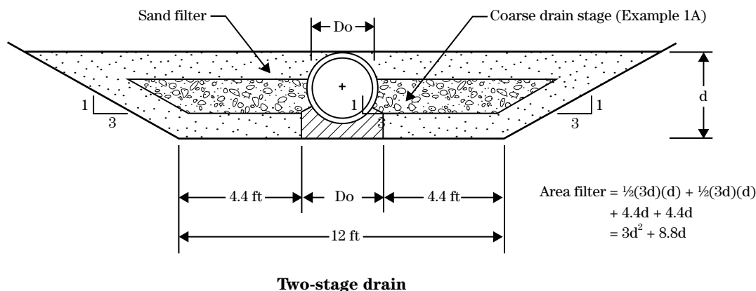
Figure 45C-4 Two-stage drain
