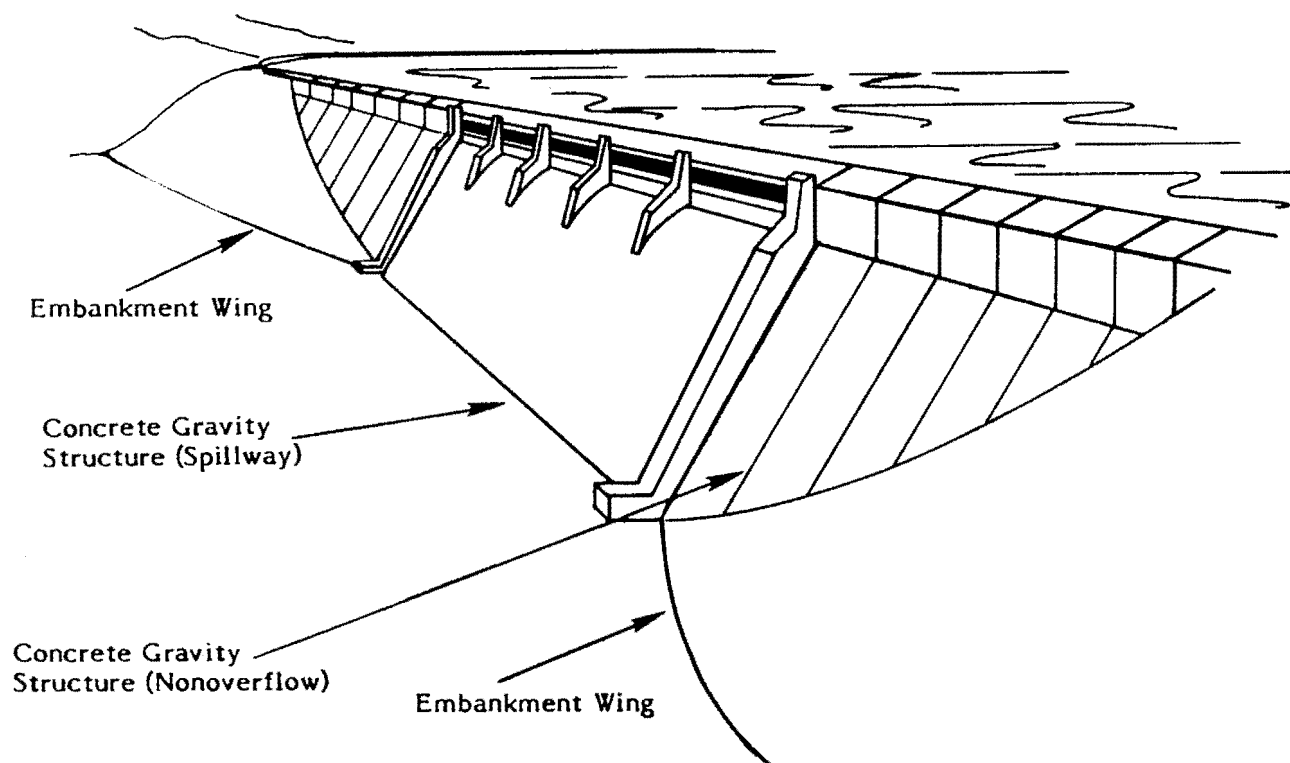
FIGURE I-4. COMPOSITE DAM
