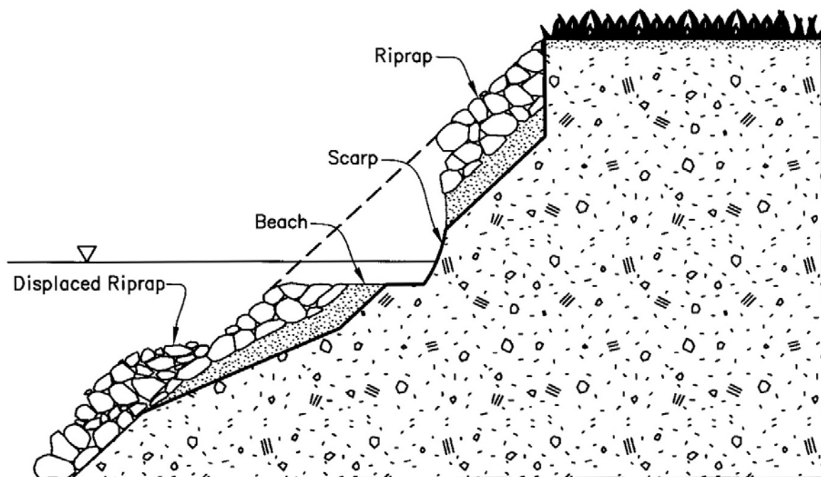
FIGURE II-15. WAVE EROSION
