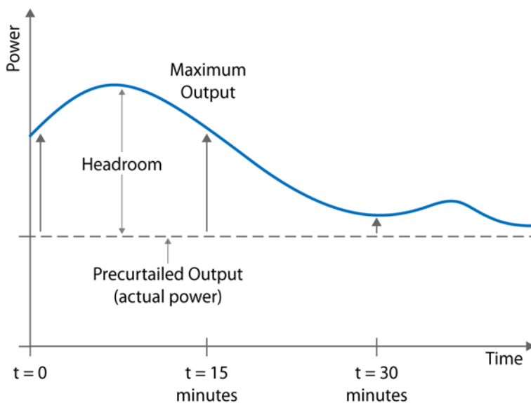
Figure 9. The impact of variable output on the ability of wind to provide upward reserve services.
