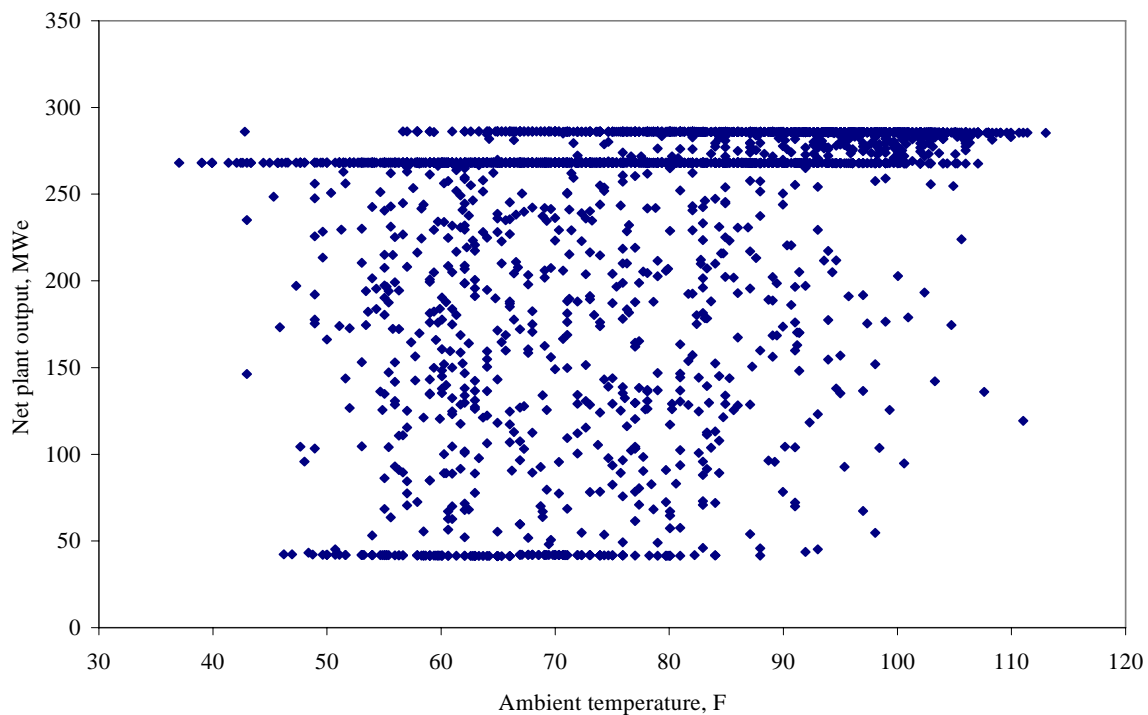
Figure 4 Net Plant Output as a Function of Ambient Temperature; Wet Heat Rejection
