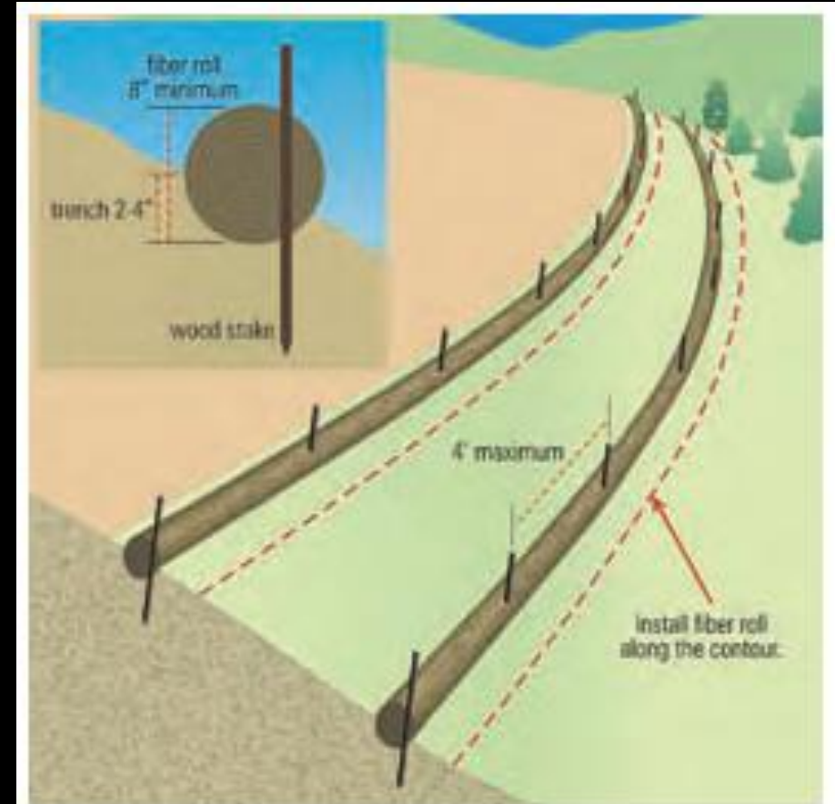
Figure 10. Illustration of a fiber roll installation along a slope
