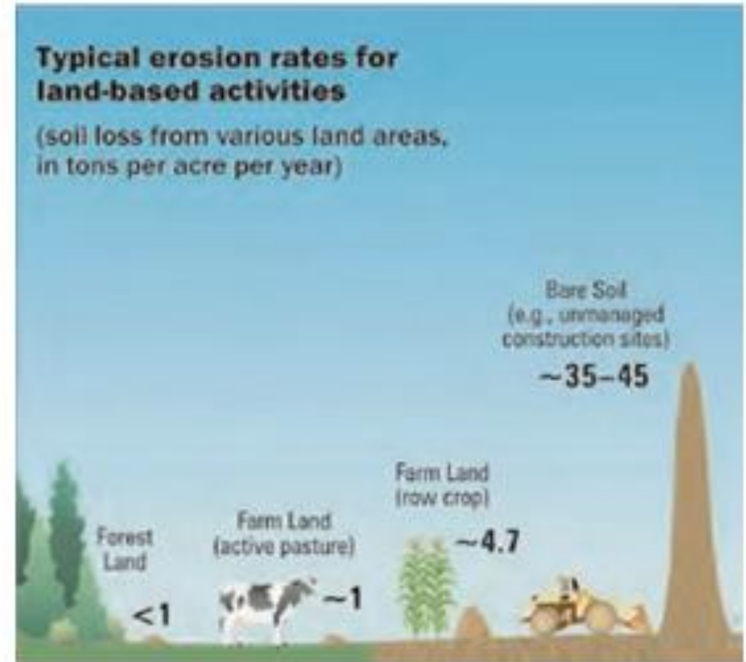
Figure 2. Typical erosion rates from land-based activities (Dunne, T. and L. Leopold, 1978; NCRS, 2000; NCRS, 2006; ASCE and WEF, 1992)
