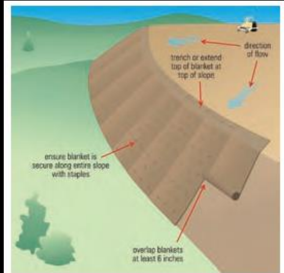
Figure 9. Illustration of erosion control blankets installed on slope
