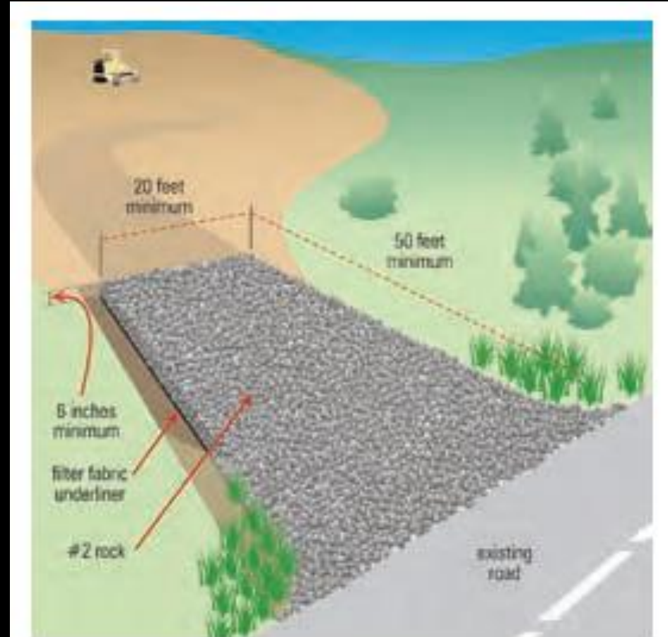
Figure 14. Illustration of a stabilized construction exit
