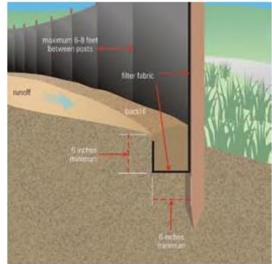
Figure 12. Illustration of proper technique to use in installing silt fence
