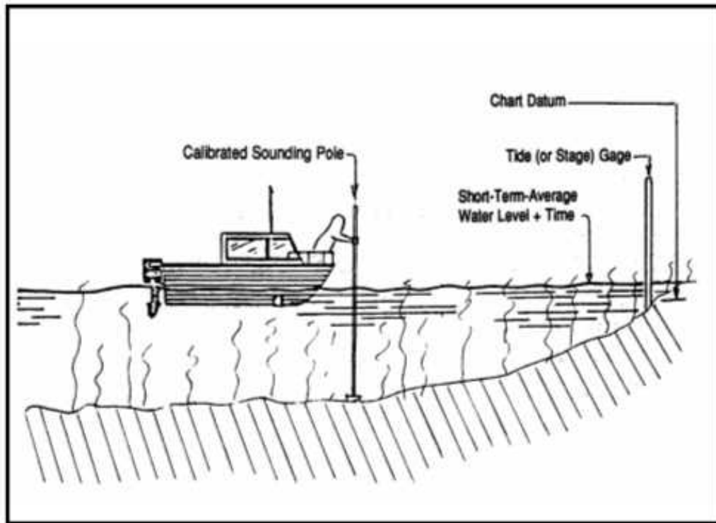
Figure B-4. Sounding pole depth measurement
