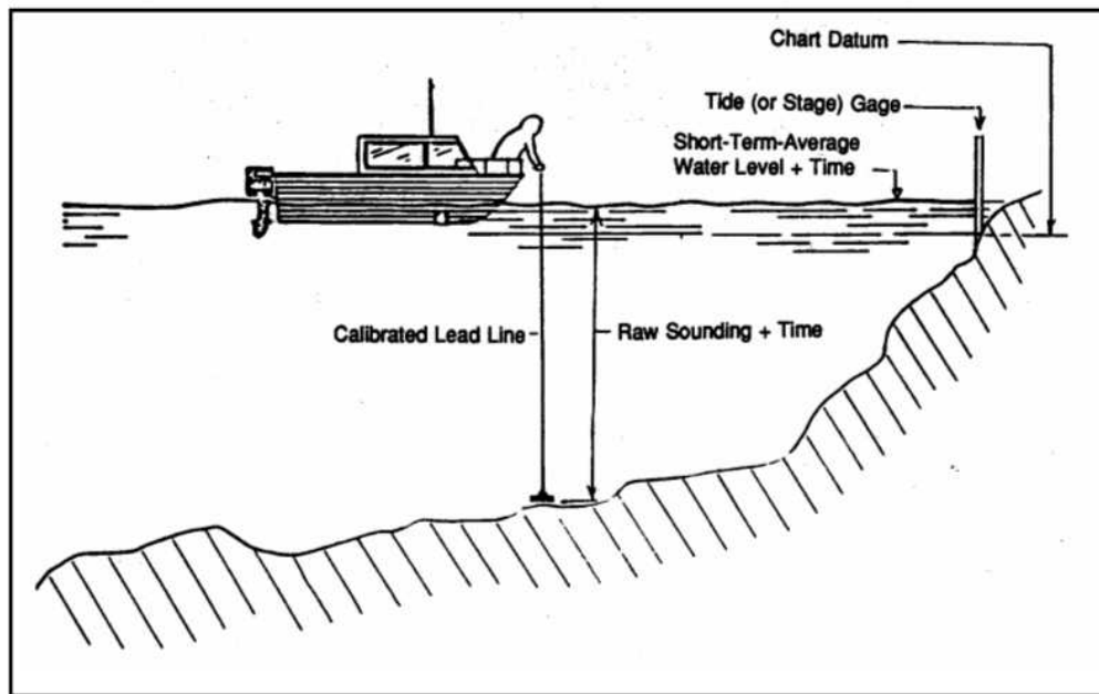
Figure B-1. Lead-line depth measurement
