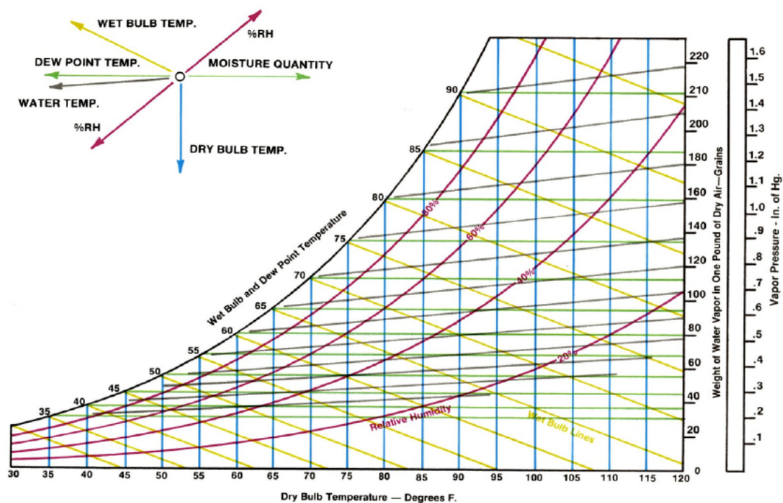
Figure 3. Psychrometric chart
