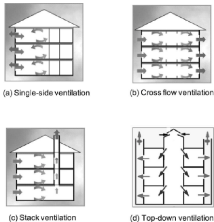
Figure 5. Types of Natural Ventilation
