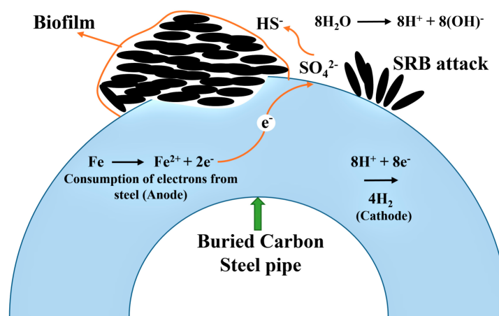
Figure 4: A schematic view of the function of sulfate-reducing bacteria (SRB) in microbiologically induced corrosion (MIC). Credit: Kiani et al., 2019.
