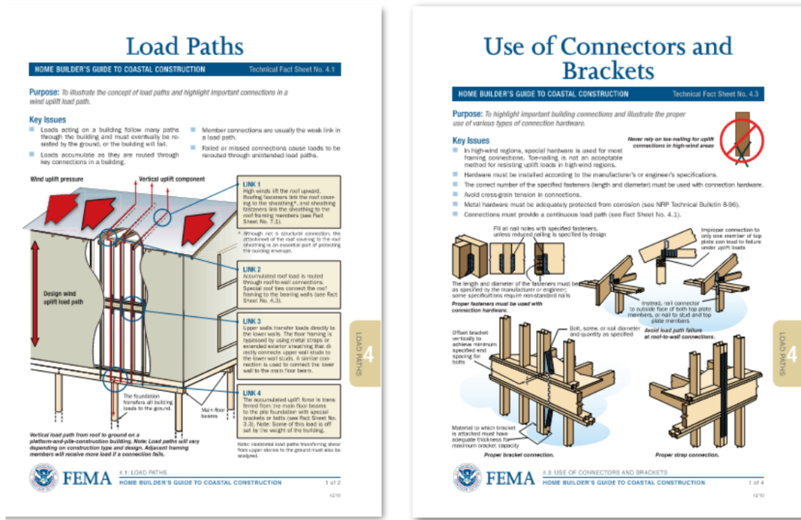
Figure 8. FEMA P-499 Technical Fact Sheets No. 4.1, Load Paths and No. 4.3, Use of Connectors and Brackets (Source: FEMA P-804)
