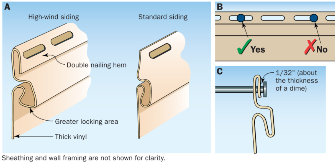
Figure 5. Fastening for high-wind vinyl siding (Source: FEMA P-499 Technical Fact Sheet 5.3, Siding Installation in High-Wind Regions)
